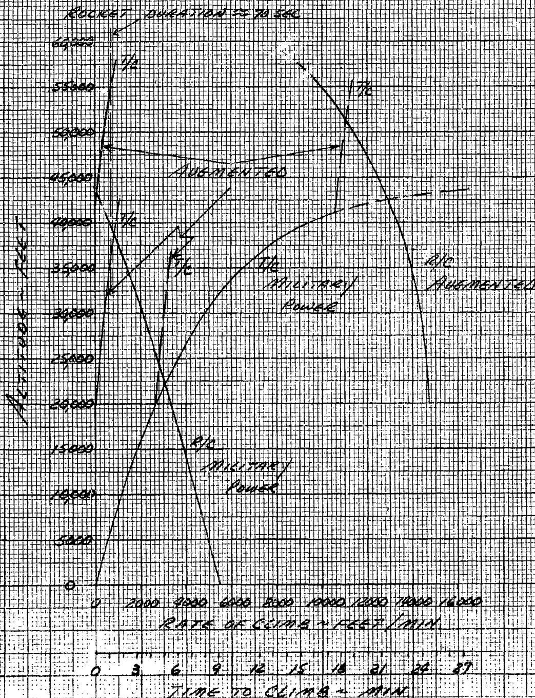
FIGURE No 3 COMBINED CLIMB PERFORMANCE F-86E USAF NO 51-2773 J-47-GE-13 ENGINE YLR 63-A1-3 ROCKET ENGINE 15,984 LBS AT ENGINE START INLET SCREENS IN PLACE
